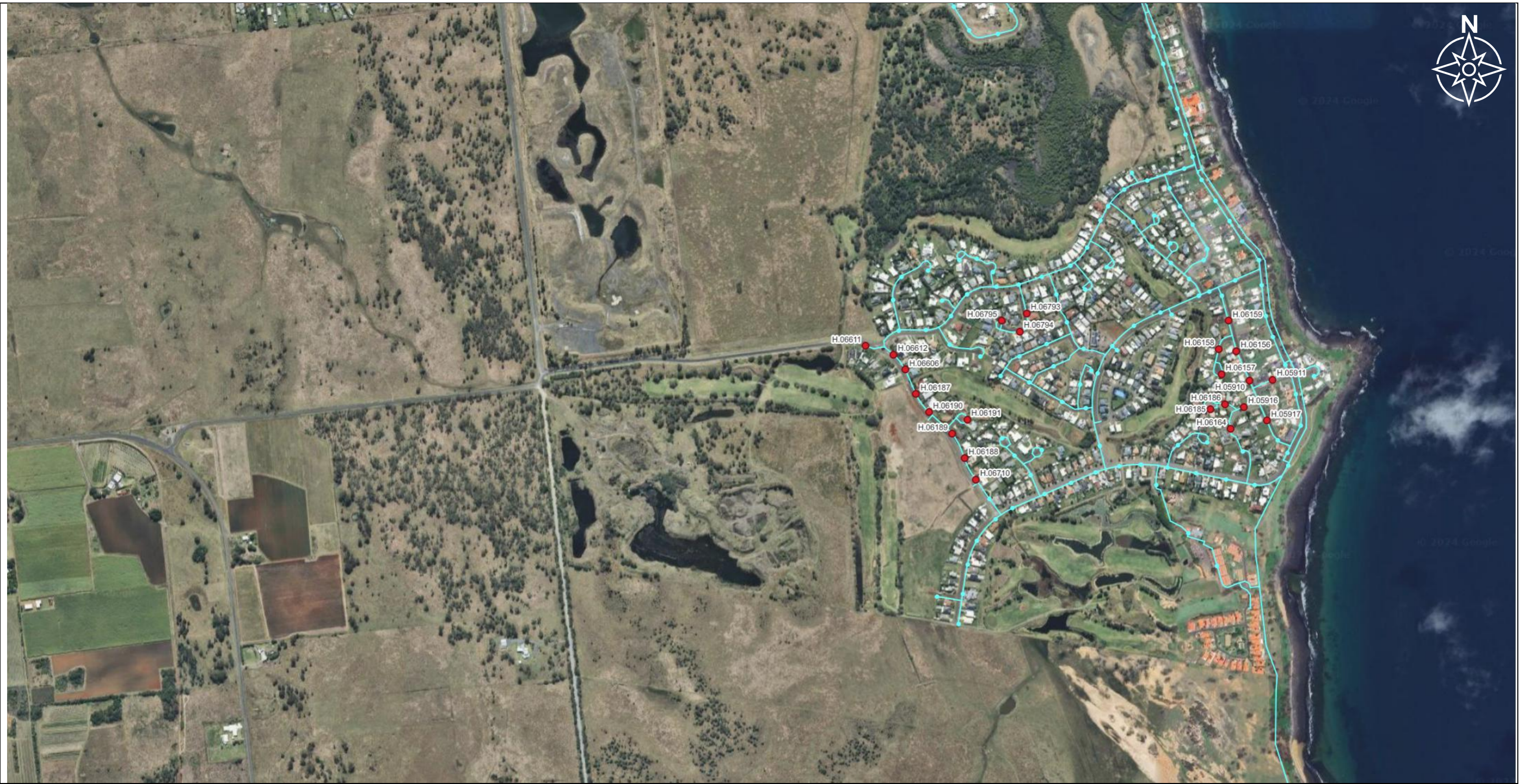
CORAL COVE HYDRANT FLOW TESTING PLAN SHEET 1 OF 1
